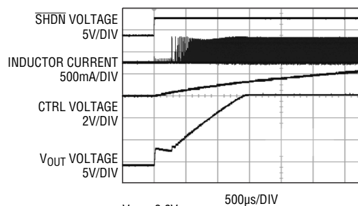
Figure 5. Soft-Start Waveform
